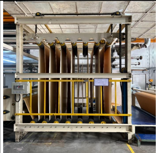
Machinery Name: 35mAccumulator Location In Plant: Main Plant Use: To Accumulate paper for continuous Process
